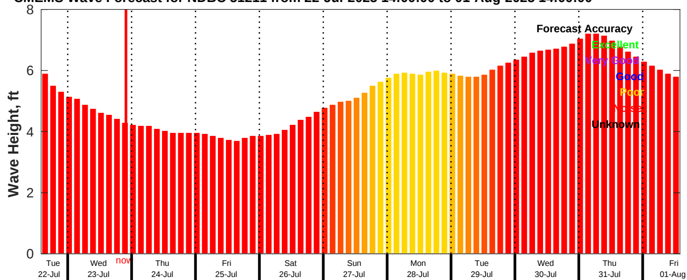
CMEMS Wave Forecast for NDBC 51211 from 22-Jul-2025 14:00:00 to 01-Aug-2025 14:00:00
