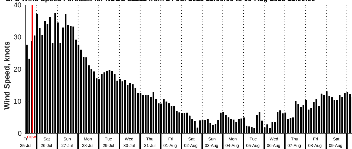
GFS Wind Speed Forecast for NDBC 52211 from 24-Jul-2025 11:00:00 to 09-Aug-2025 11:00:00
