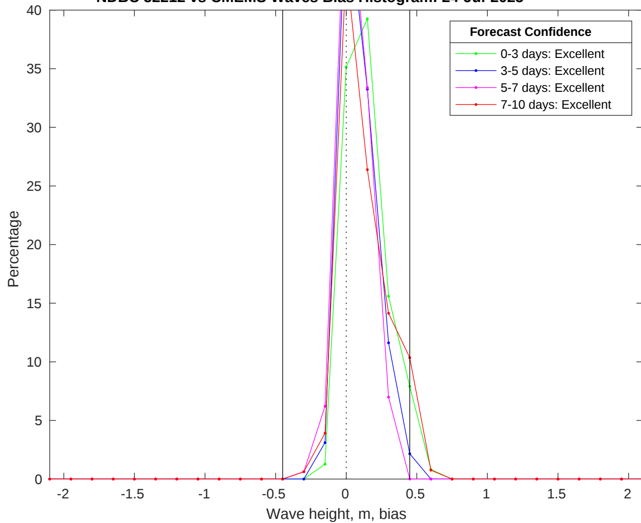
NDBC 52212 vs CMEMS Waves Bias Histogram: 24-Jul-2025
