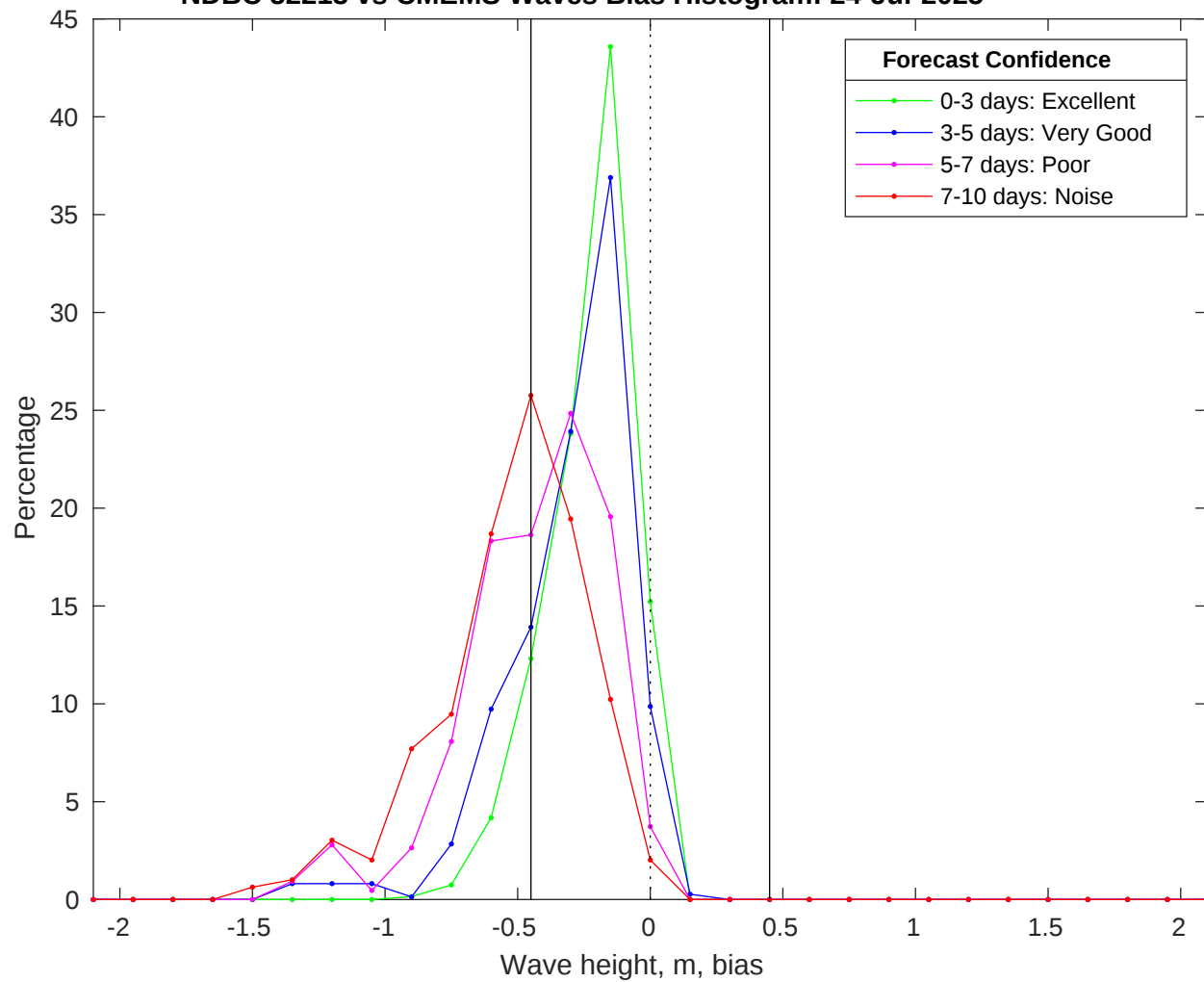
NDBC 52213 vs CMEMS Waves Bias Histogram: 24-Jul-2025
