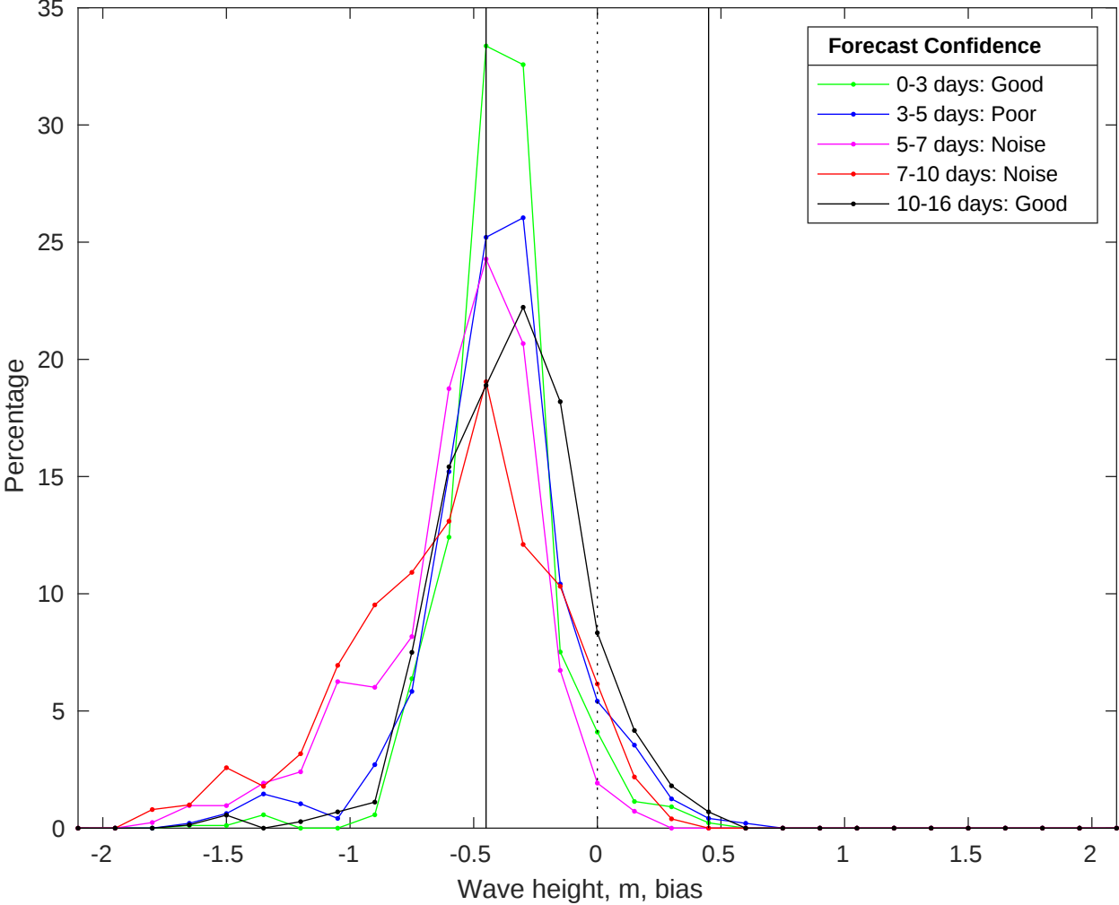
NDBC 52213 vs GFS Waves Bias Histogram: 24-Jul-2025
