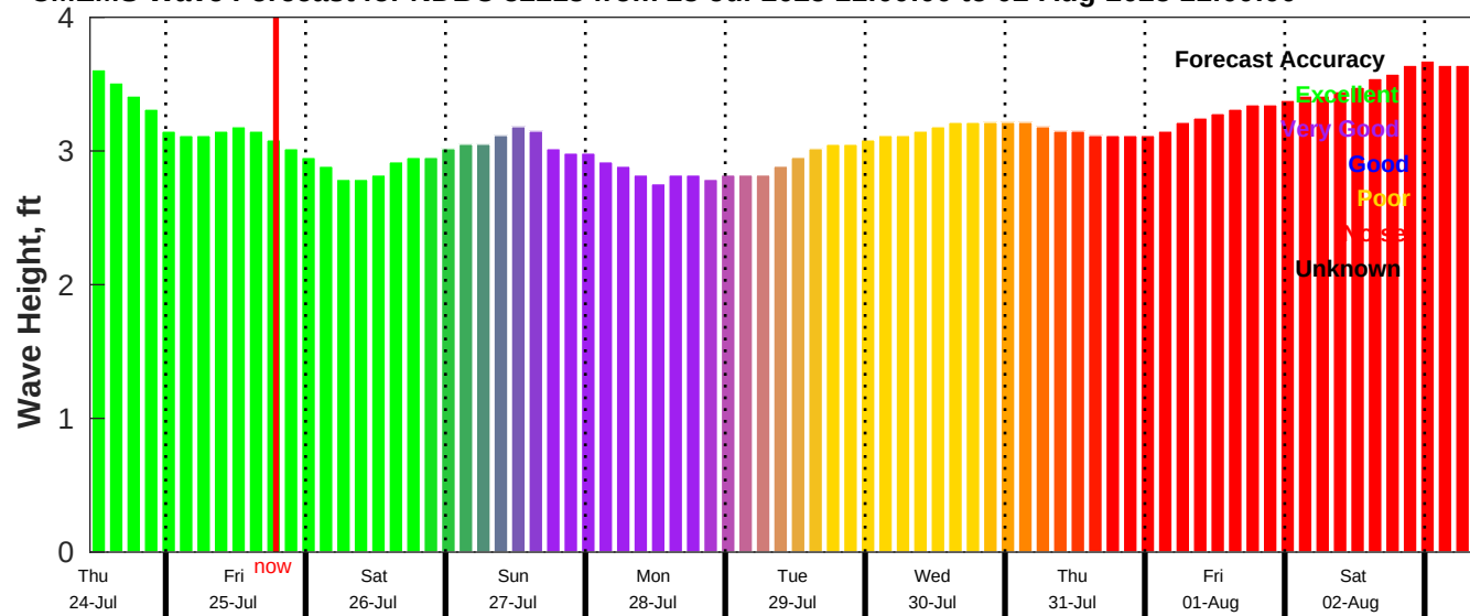
CMEMS Wave Forecast for NDBC 52213 from 23-Jul-2025 11:00:00 to 02-Aug-2025 11:00:00
