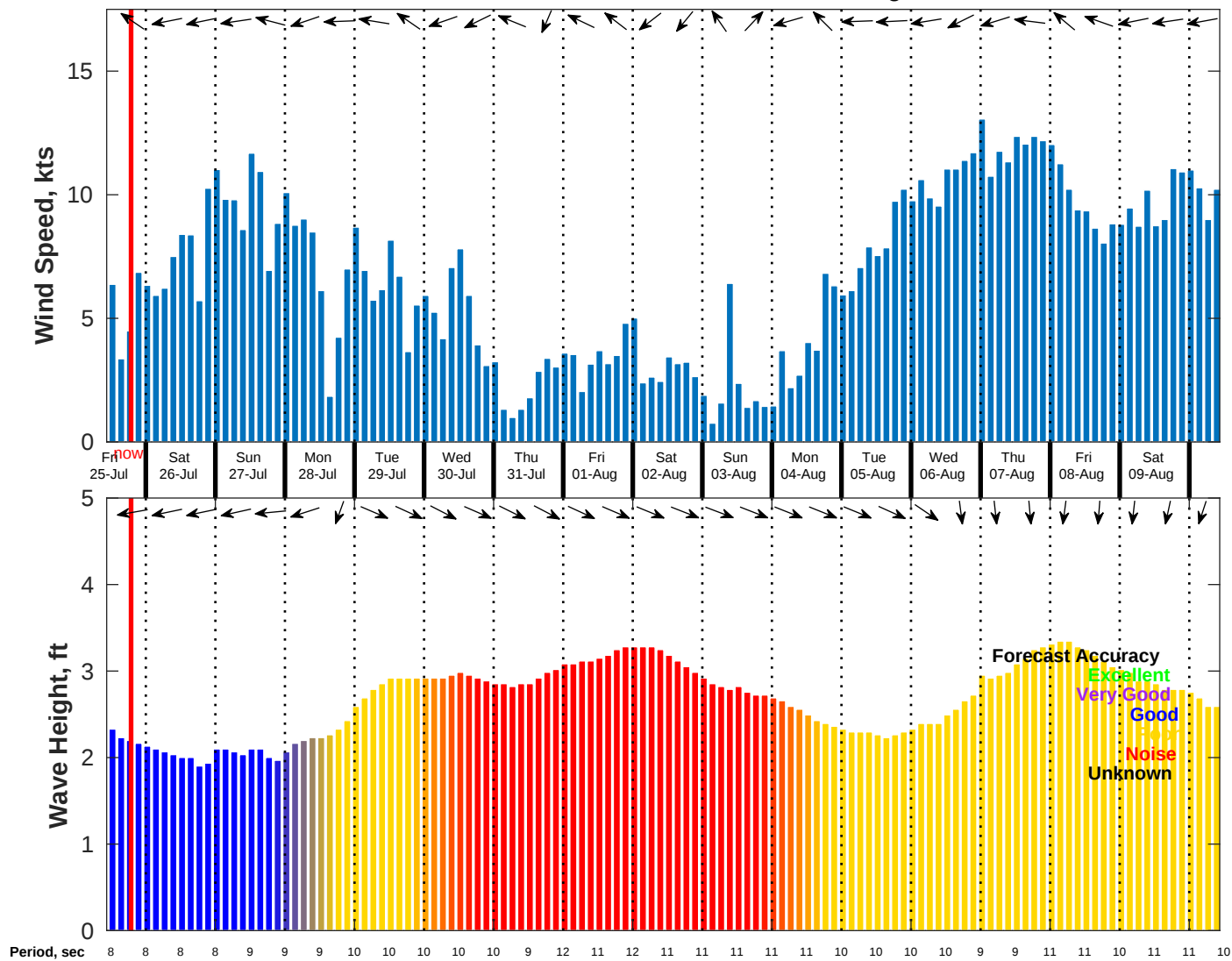
Wind & Wave Forecast for NDBC 52213 from 24-Jul-2025 11:00:00 to 09-Aug-2025 11:00:00
