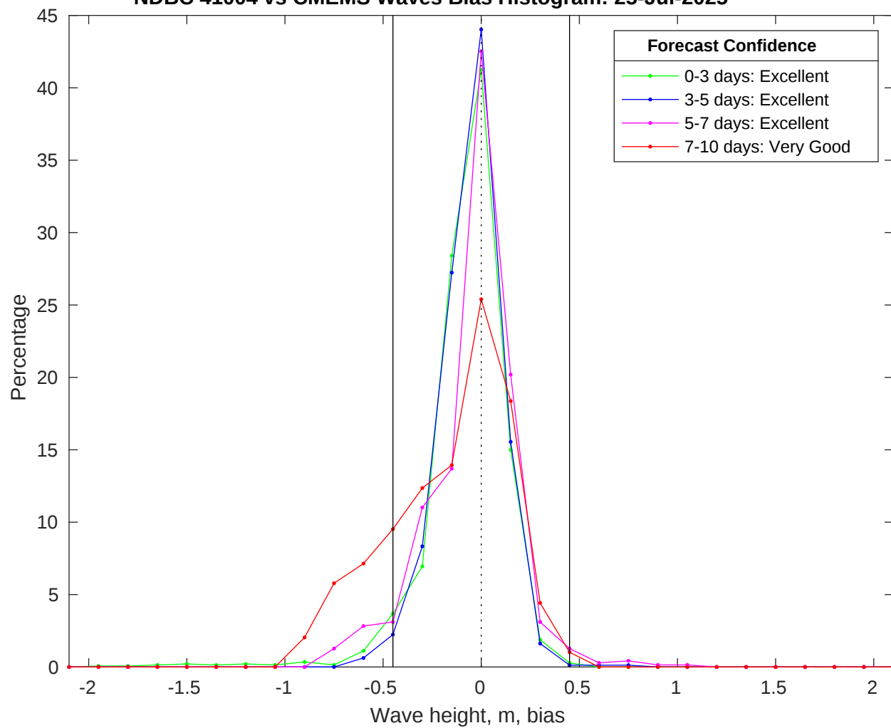
NDBC 41004 vs CMEMS Waves Bias Histogram: 25-Jul-2025
