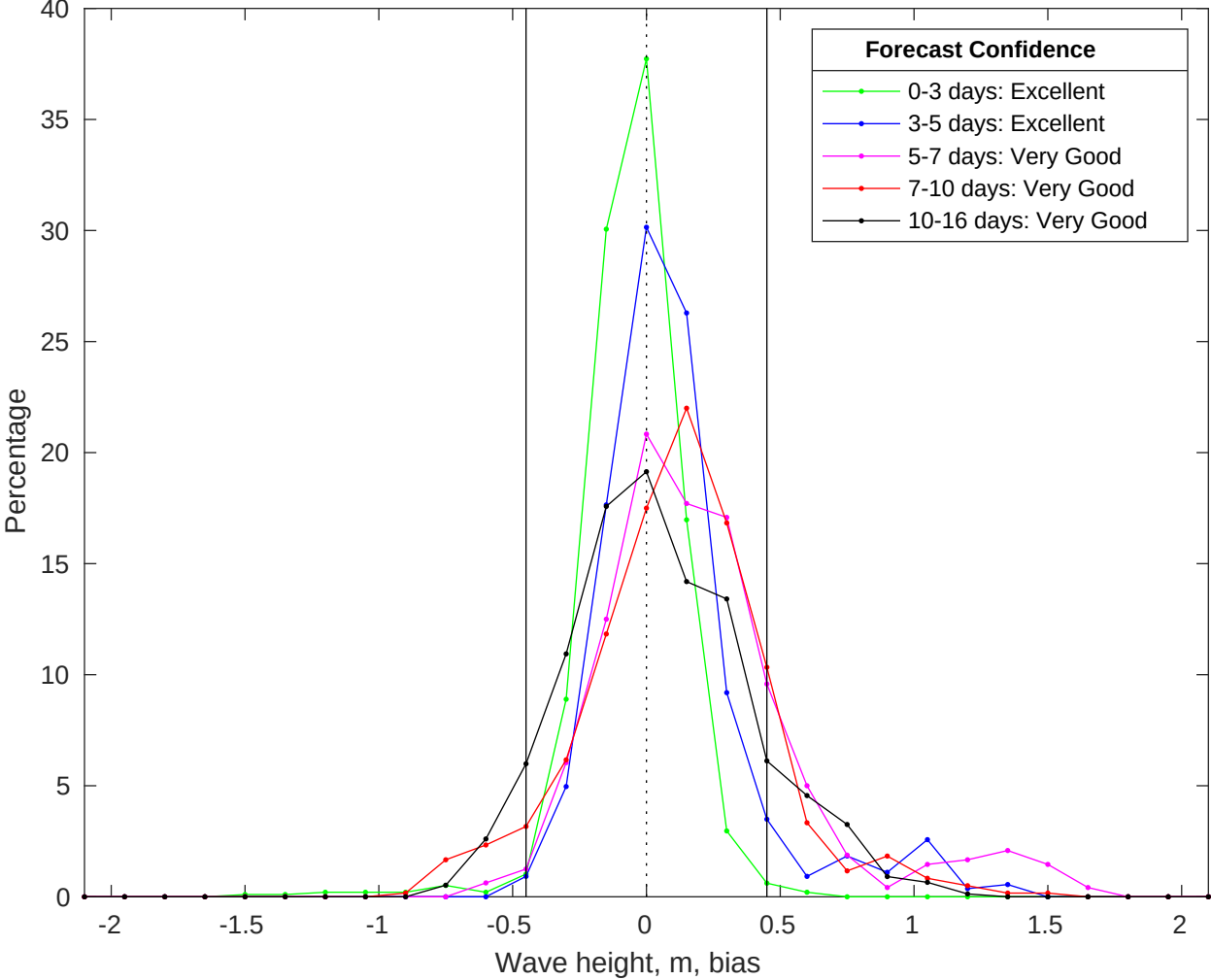
NDBC 41004 vs GFS Waves Bias Histogram: 25-Jul-2025
