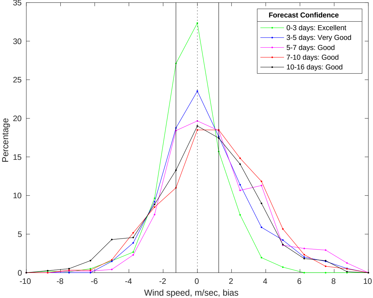
NDBC 41004 vs GFS Winds Bias Histogram: 25-Jul-2025
