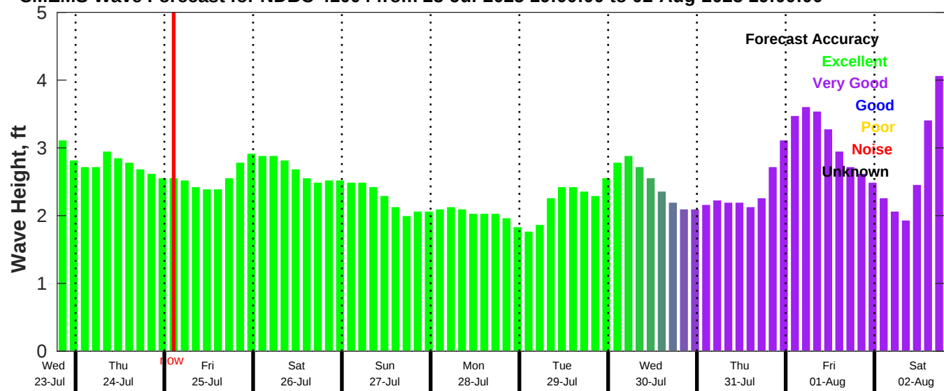
CMEMS Wave Forecast for NDBC 41004 from 23-Jul-2025 19:00:00 to 02-Aug-2025 19:00:00
