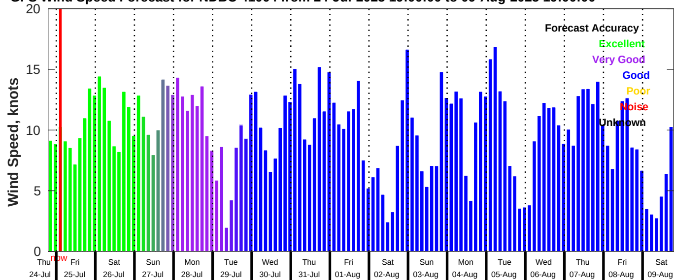
GFS Wind Speed Forecast for NDBC 41004 from 24-Jul-2025 19:00:00 to 09-Aug-2025 19:00:00
