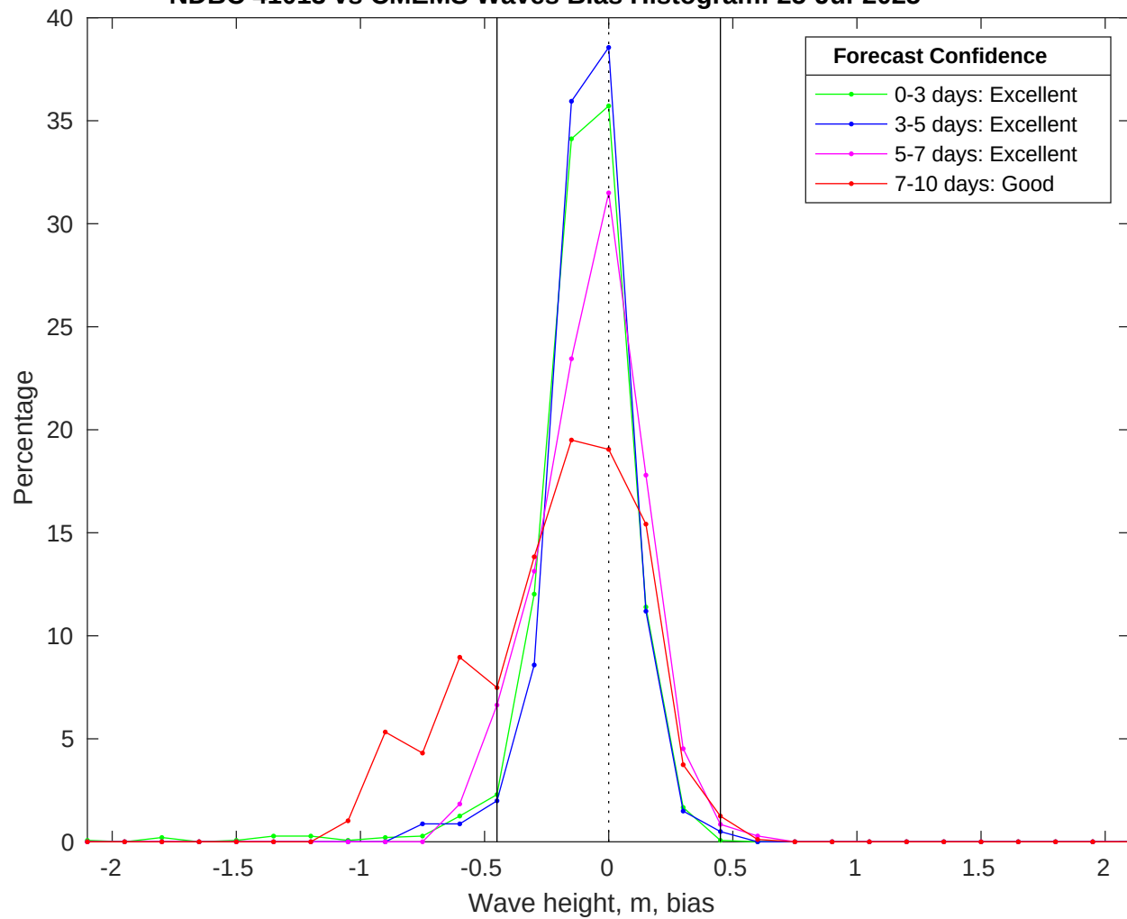
NDBC 41013 vs CMEMS Waves Bias Histogram: 25-Jul-2025
