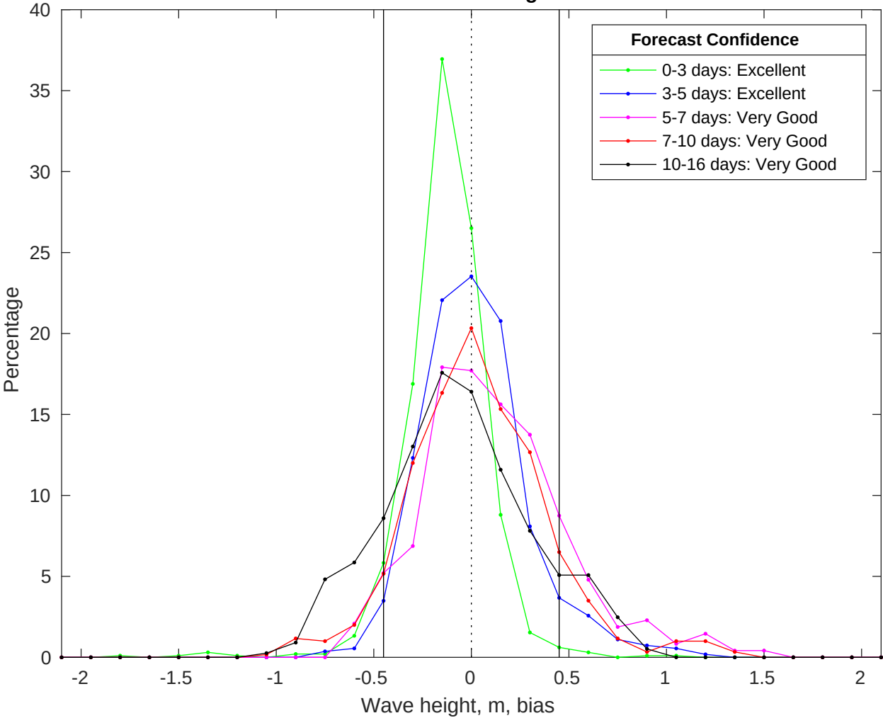
NDBC 41013 vs GFS Waves Bias Histogram: 25-Jul-2025
