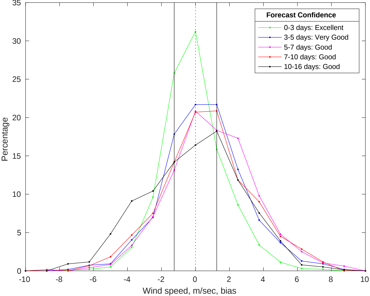
NDBC 41013 vs GFS Winds Bias Histogram: 25-Jul-2025
