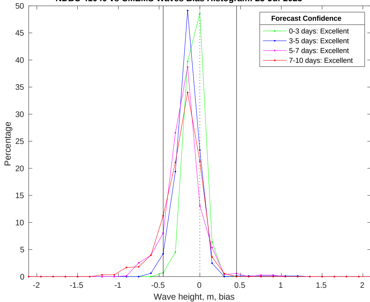
NDBC 41040 vs CMEMS Waves Bias Histogram: 25-Jul-2025
