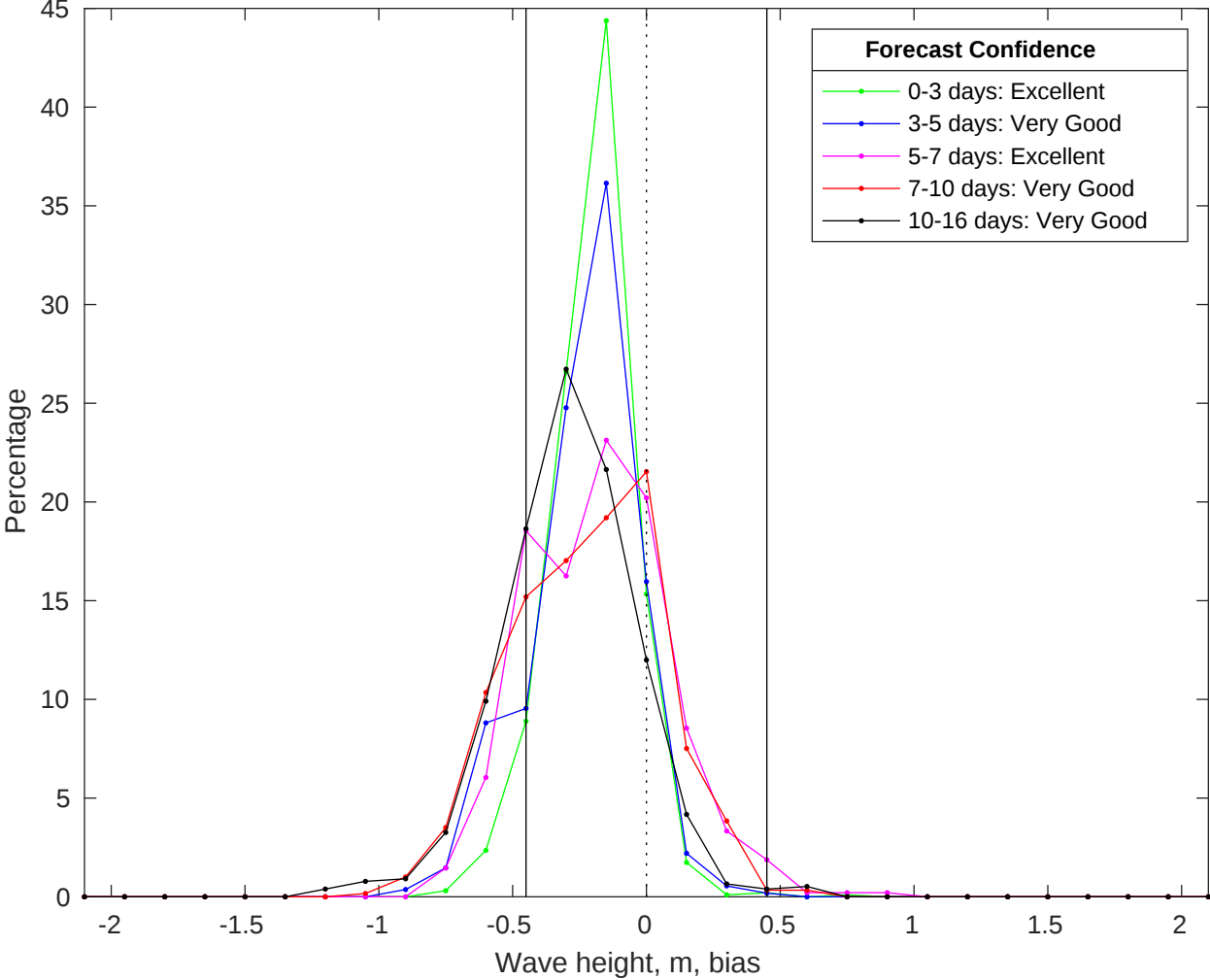
NDBC 41040 vs GFS Waves Bias Histogram: 25-Jul-2025
