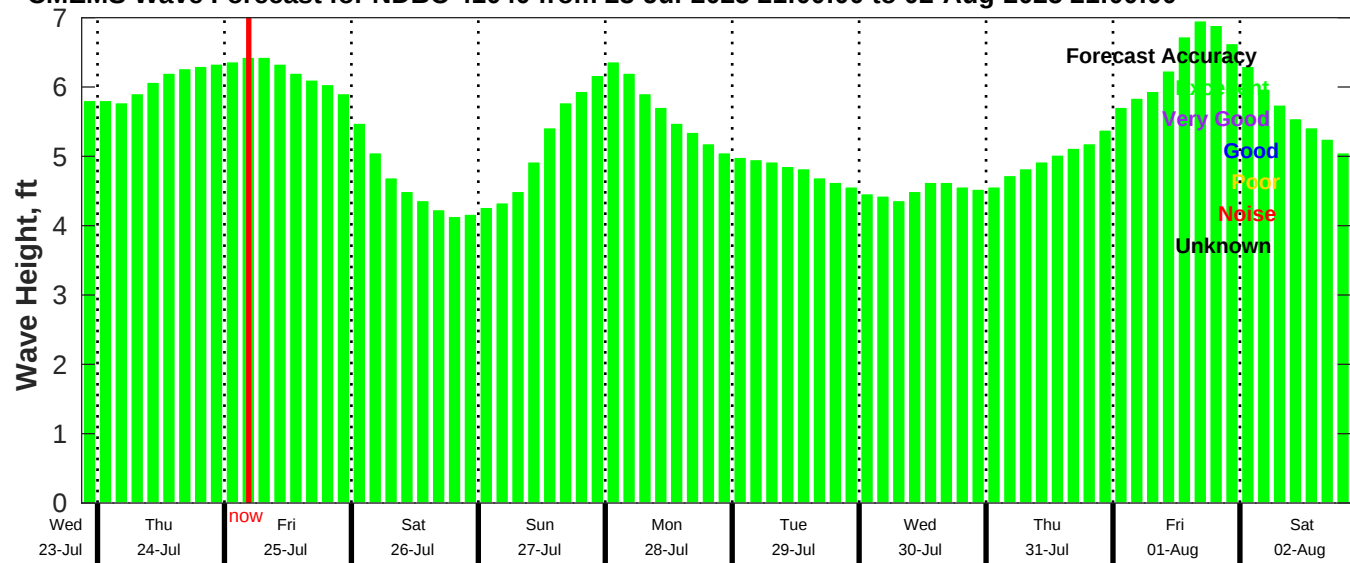
CMEMS Wave Forecast for NDBC 41040 from 23-Jul-2025 21:00:00 to 02-Aug-2025 21:00:00
