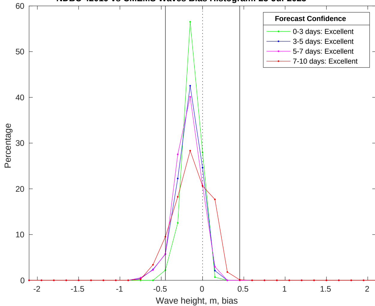
NDBC 42019 vs CMEMS Waves Bias Histogram: 25-Jul-2025
