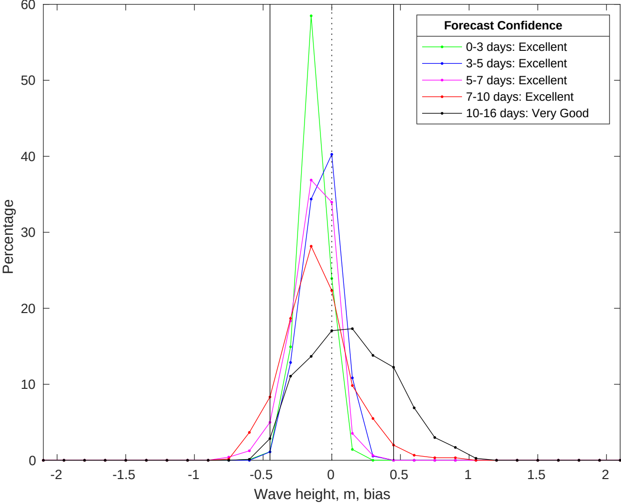
NDBC 42019 vs GFS Waves Bias Histogram: 25-Jul-2025
