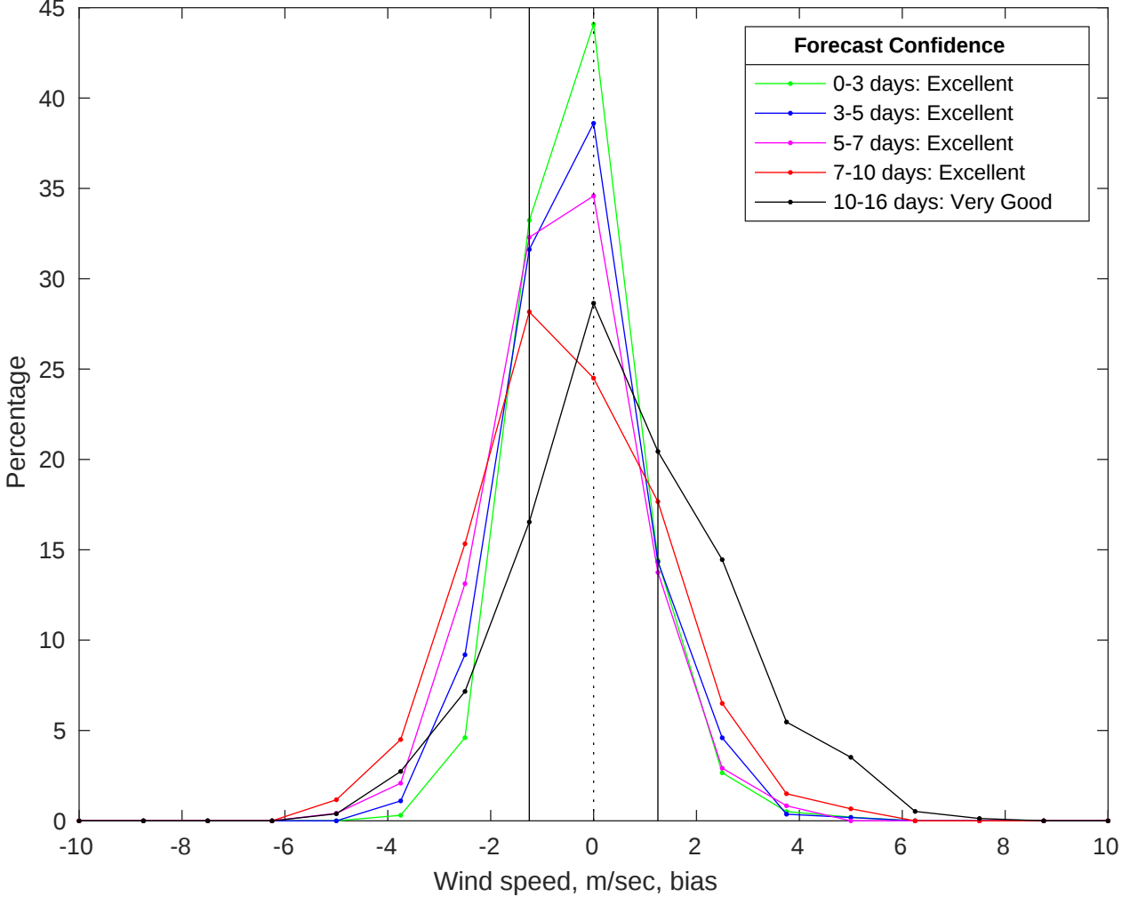
NDBC 42019 vs GFS Winds Bias Histogram: 25-Jul-2025
