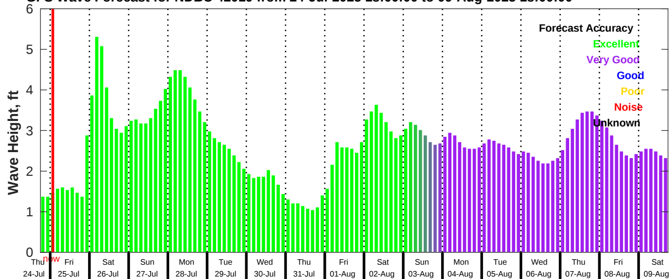
GFS Wave Forecast for NDBC 42019 from 24-Jul-2025 18:00:00 to 09-Aug-2025 18:00:00
