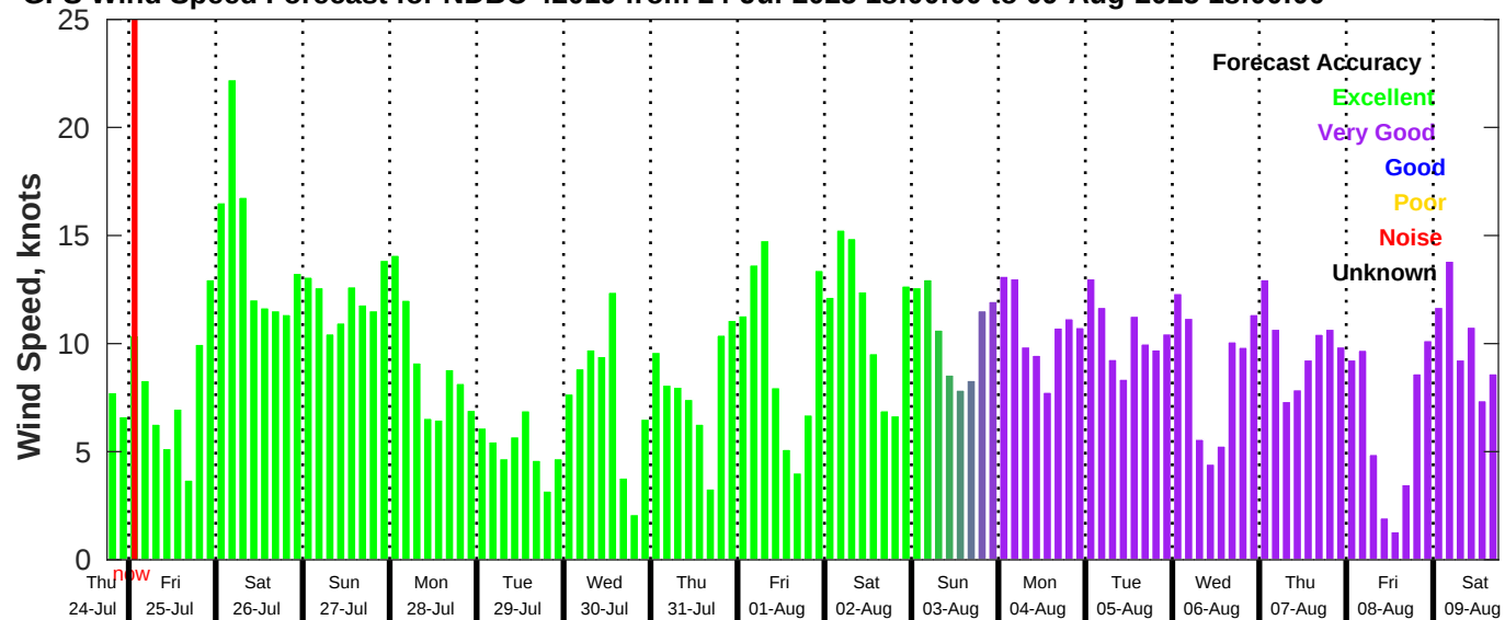
GFS Wind Speed Forecast for NDBC 42019 from 24-Jul-2025 18:00:00 to 09-Aug-2025 18:00:00
