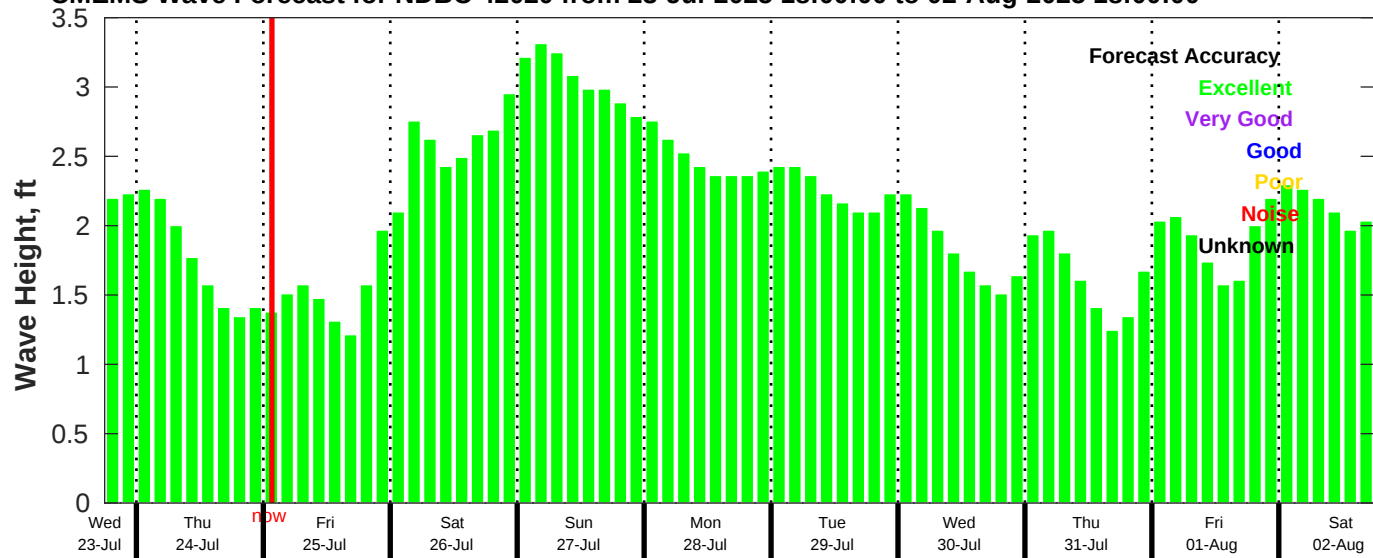
CMEMS Wave Forecast for NDBC 42020 from 23-Jul-2025 18:00:00 to 02-Aug-2025 18:00:00
