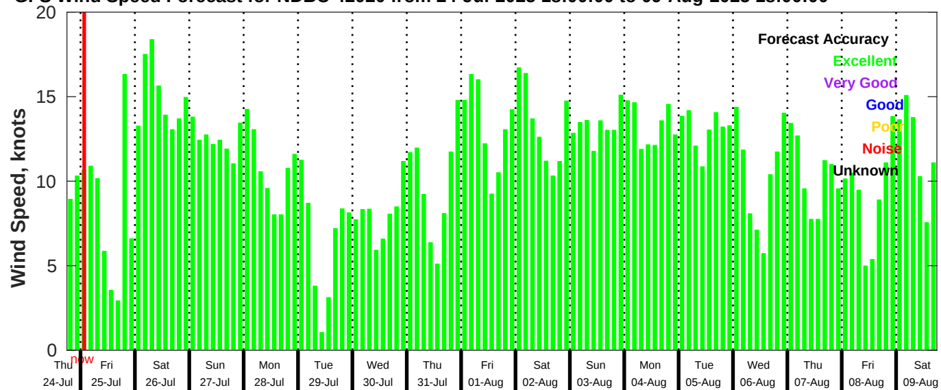
GFS Wind Speed Forecast for NDBC 42020 from 24-Jul-2025 18:00:00 to 09-Aug-2025 18:00:00
