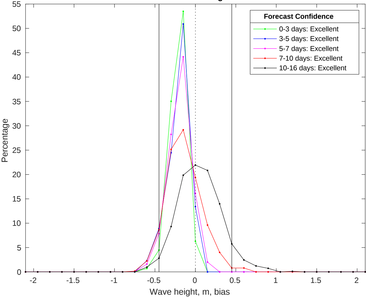
NDBC 42035 vs GFS Waves Bias Histogram: 25-Jul-2025
