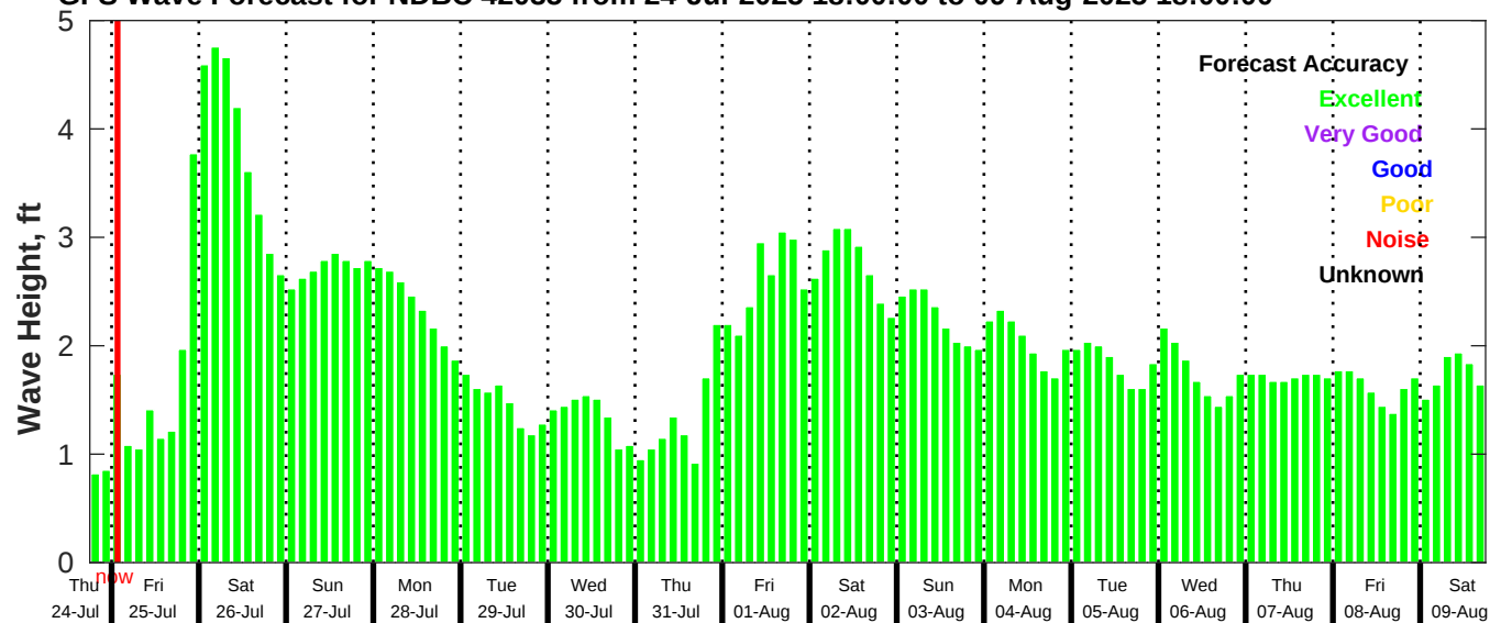
GFS Wave Forecast for NDBC 42035 from 24-Jul-2025 18:00:00 to 09-Aug-2025 18:00:00
