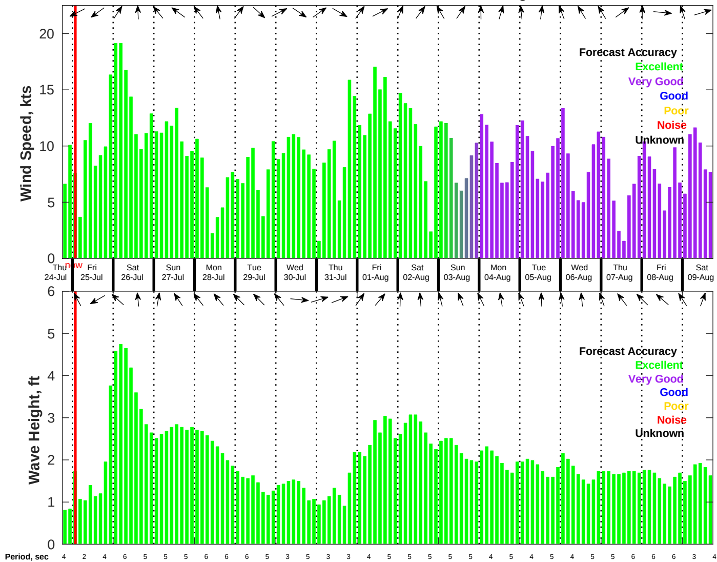
Wind & Wave Forecast for NDBC 42035 from 24-Jul-2025 18:00:00 to 09-Aug-2025 18:00:00
