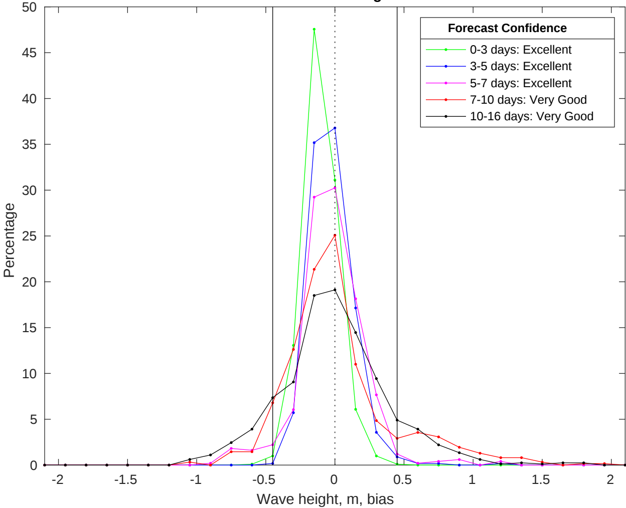
NDBC 42036 vs GFS Waves Bias Histogram: 25-Jul-2025
