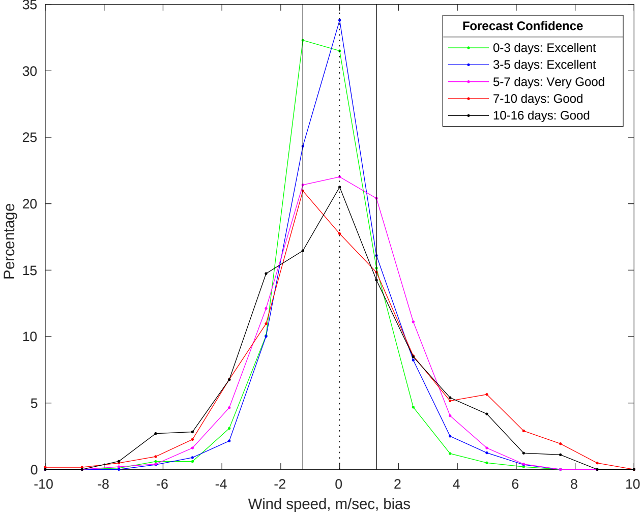
NDBC 42036 vs GFS Winds Bias Histogram: 25-Jul-2025
