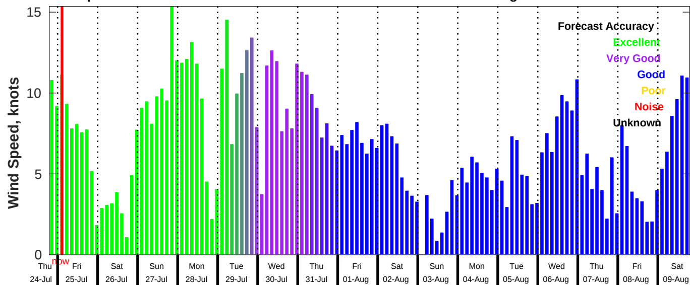
GFS Wind Speed Forecast for NDBC 42036 from 24-Jul-2025 19:00:00 to 09-Aug-2025 19:00:00
