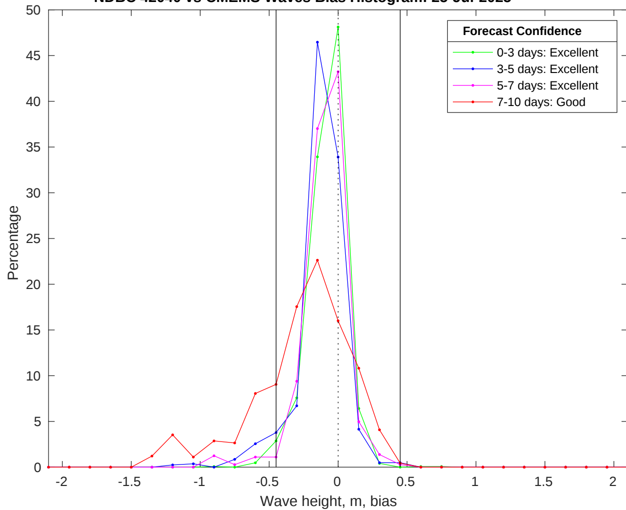
NDBC 42040 vs CMEMS Waves Bias Histogram: 25-Jul-2025
