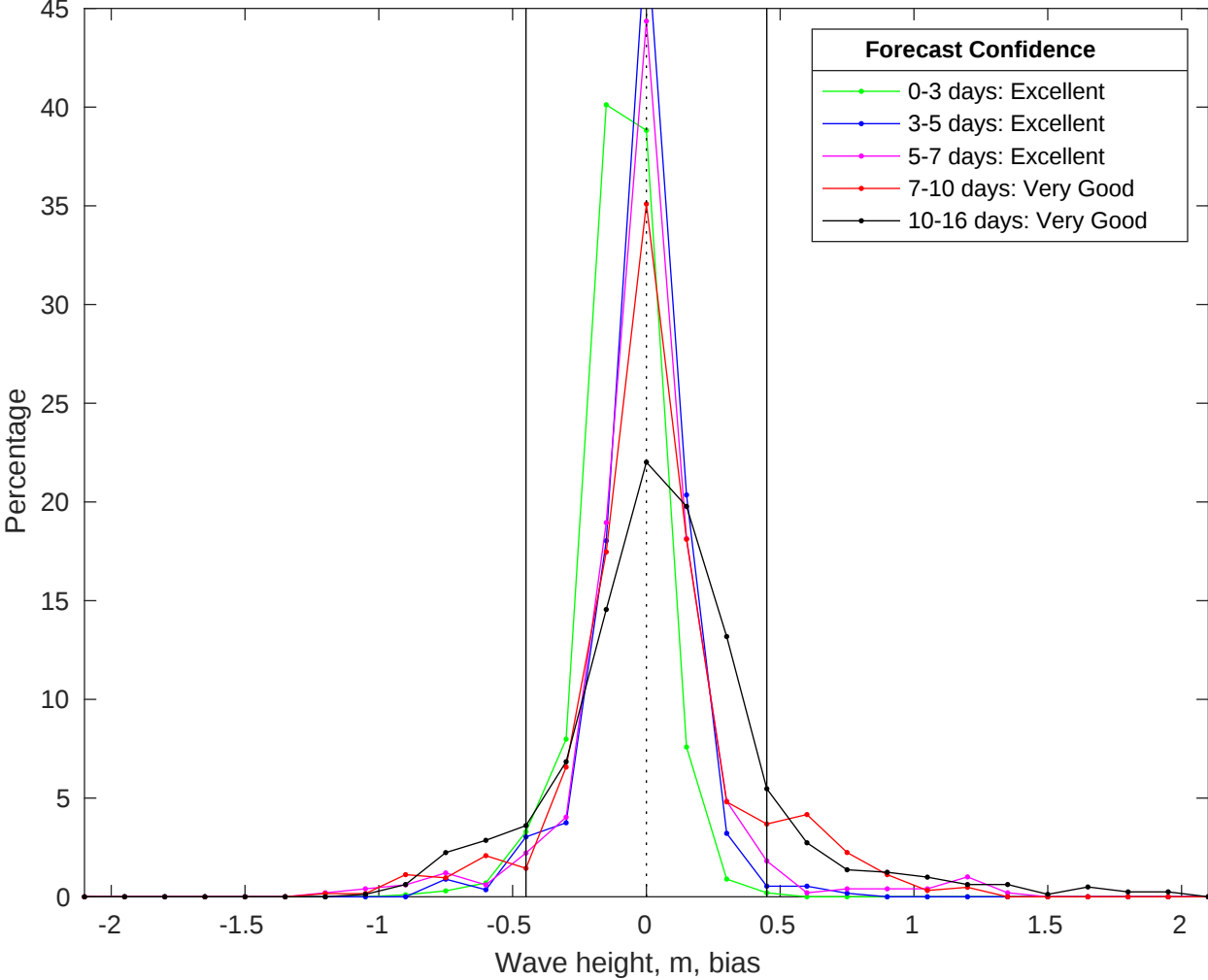
NDBC 42040 vs GFS Waves Bias Histogram: 25-Jul-2025
