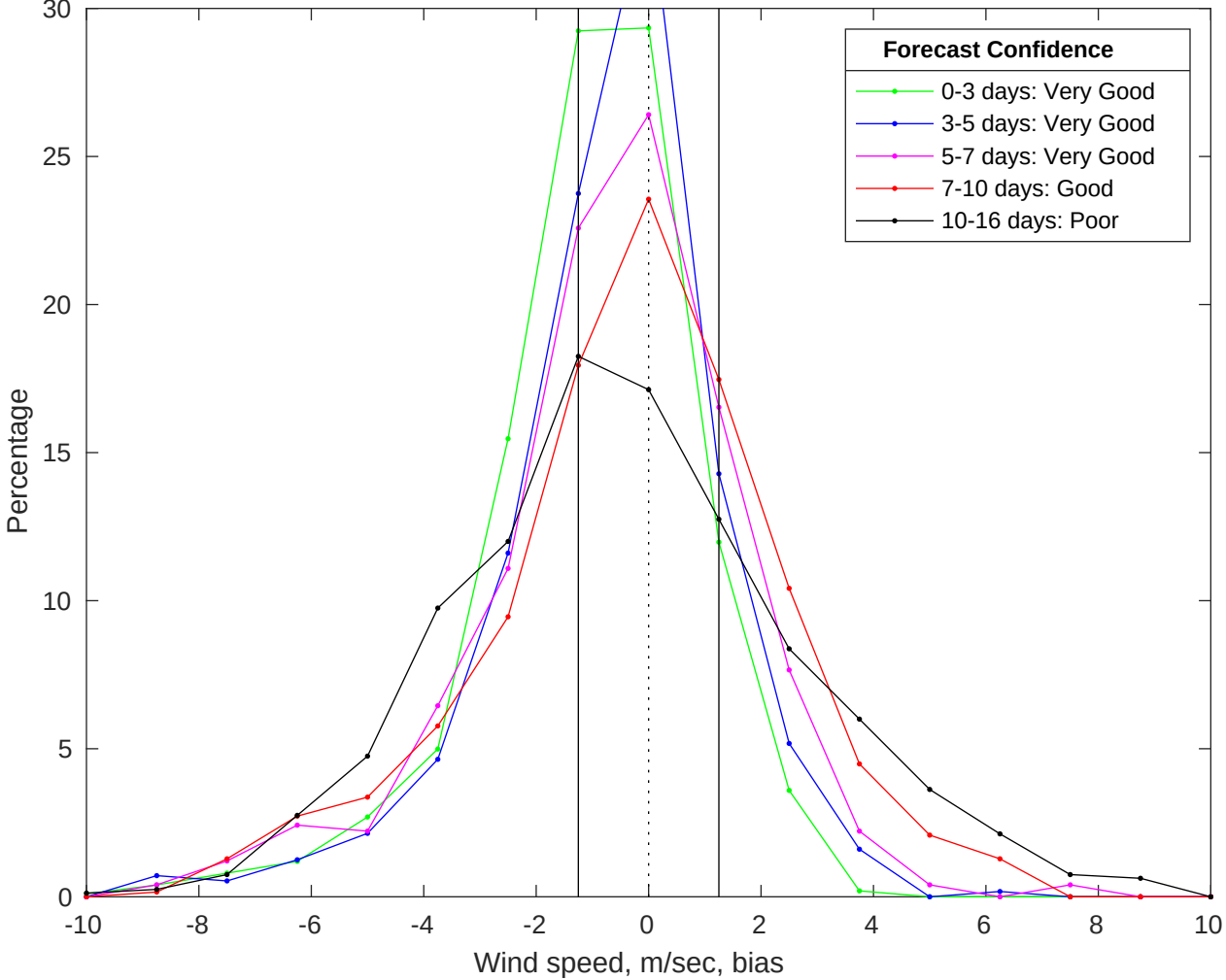
NDBC 42040 vs GFS Winds Bias Histogram: 25-Jul-2025
