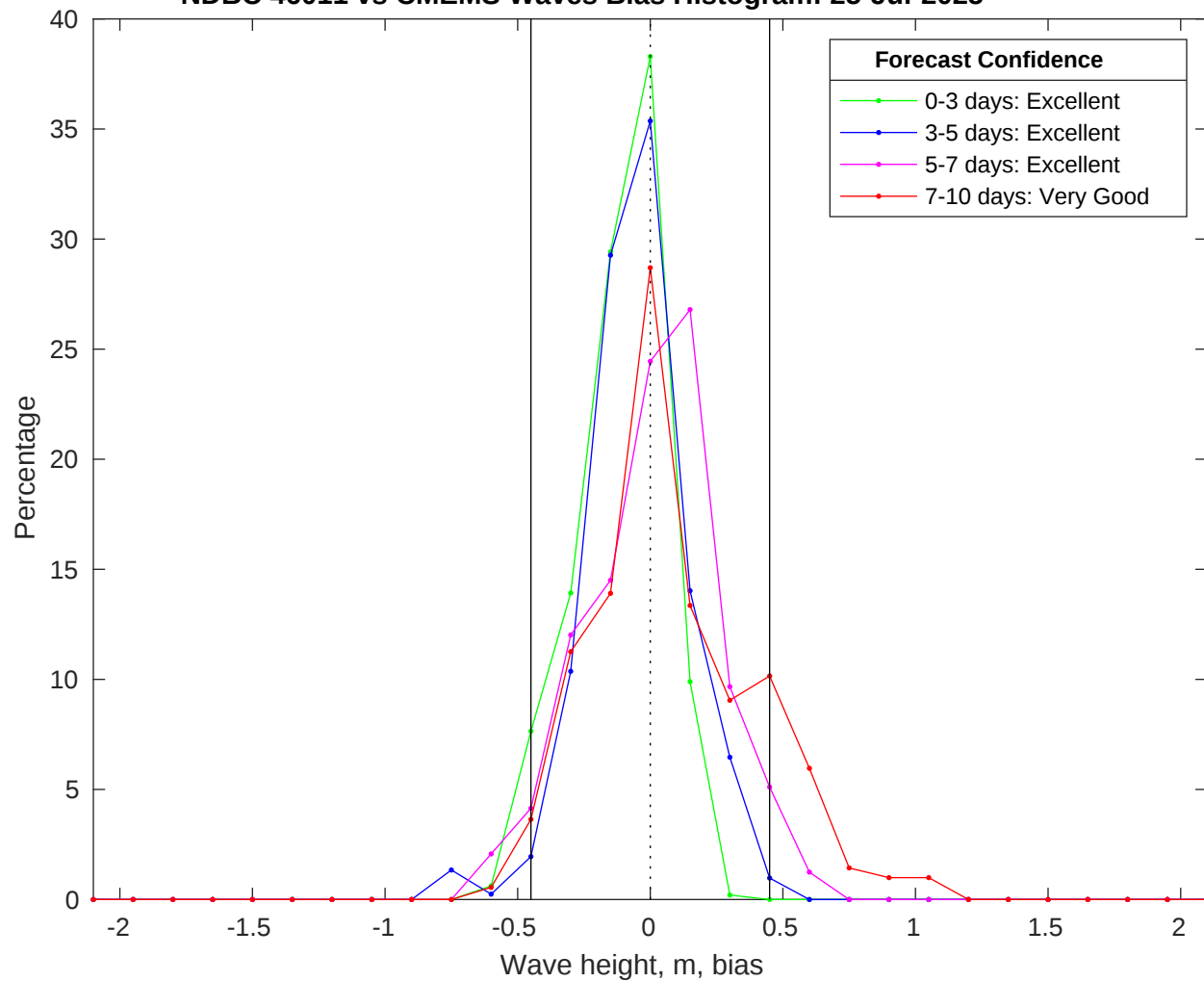
NDBC 46011 vs CMEMS Waves Bias Histogram: 25-Jul-2025
