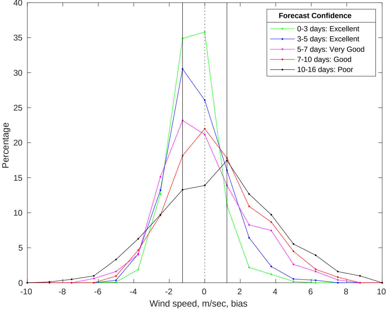
NDBC 46011 vs GFS Winds Bias Histogram: 25-Jul-2025
