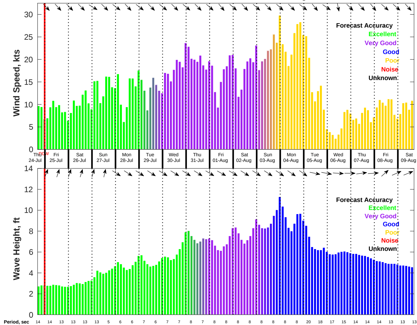
Wind & Wave Forecast for NDBC 46011 from 24-Jul-2025 16:00:00 to 09-Aug-2025 16:00:00
