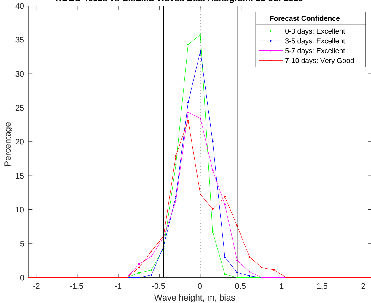
NDBC 46028 vs CMEMS Waves Bias Histogram: 25-Jul-2025
