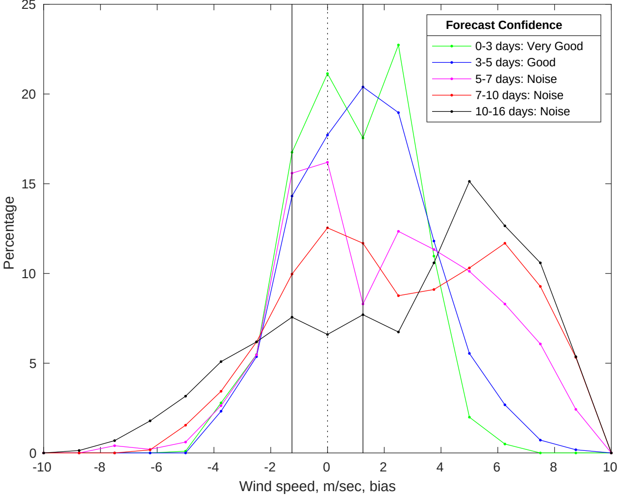
NDBC 46028 vs GFS Winds Bias Histogram: 25-Jul-2025
