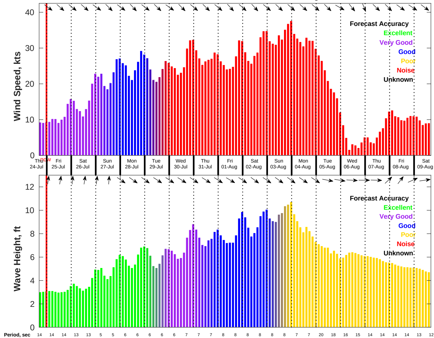
Wind & Wave Forecast for NDBC 46028 from 24-Jul-2025 16:00:00 to 09-Aug-2025 16:00:00
