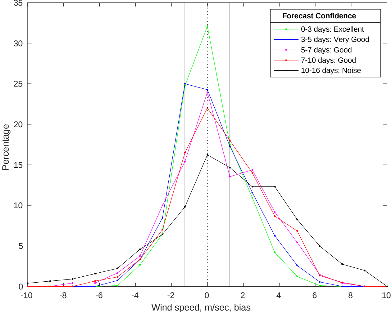
NDBC 46054 vs GFS Winds Bias Histogram: 25-Jul-2025
