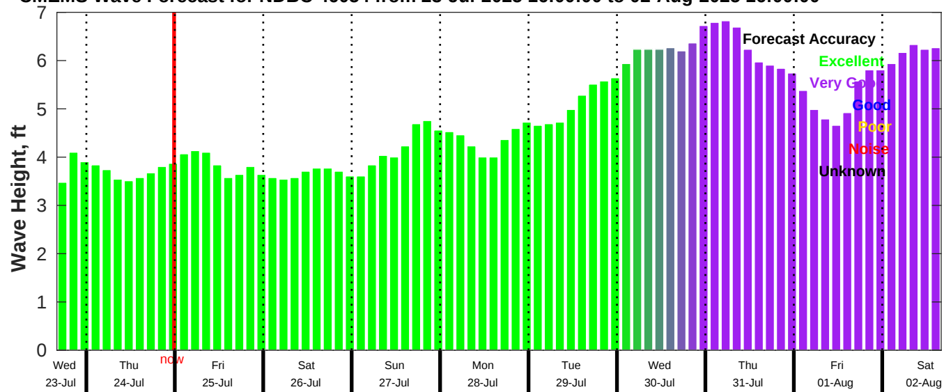
CMEMS Wave Forecast for NDBC 46054 from 23-Jul-2025 16:00:00 to 02-Aug-2025 16:00:00
