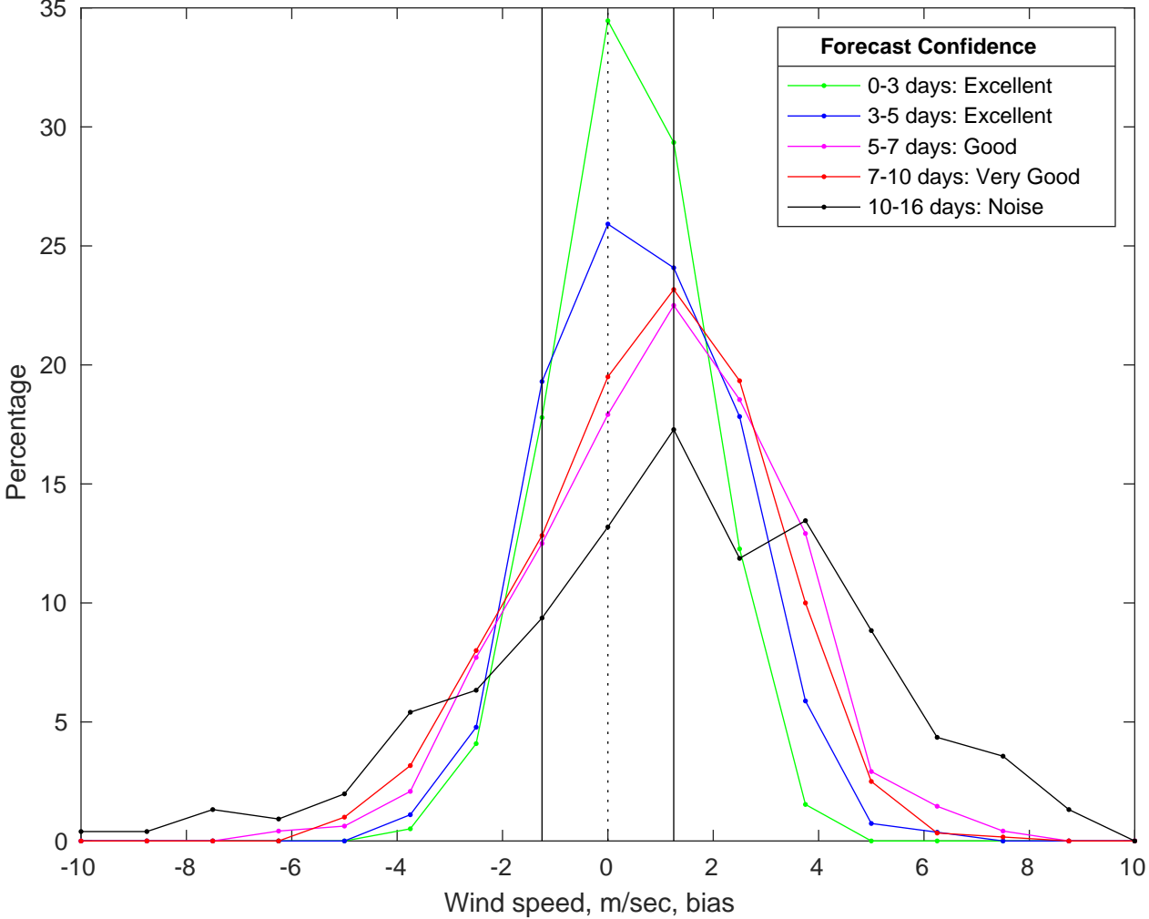
NDBC 46069 vs GFS Winds Bias Histogram: 25-Jul-2025
