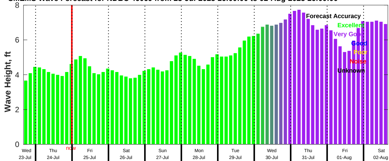
CMEMS Wave Forecast for NDBC 46069 from 23-Jul-2025 16:00:00 to 02-Aug-2025 16:00:00
