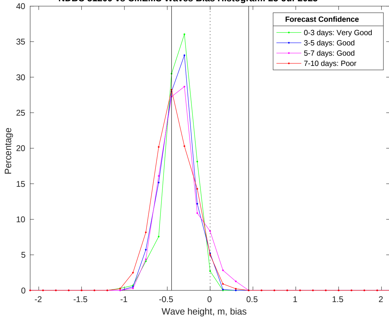
NDBC 51209 vs CMEMS Waves Bias Histogram: 25-Jul-2025
