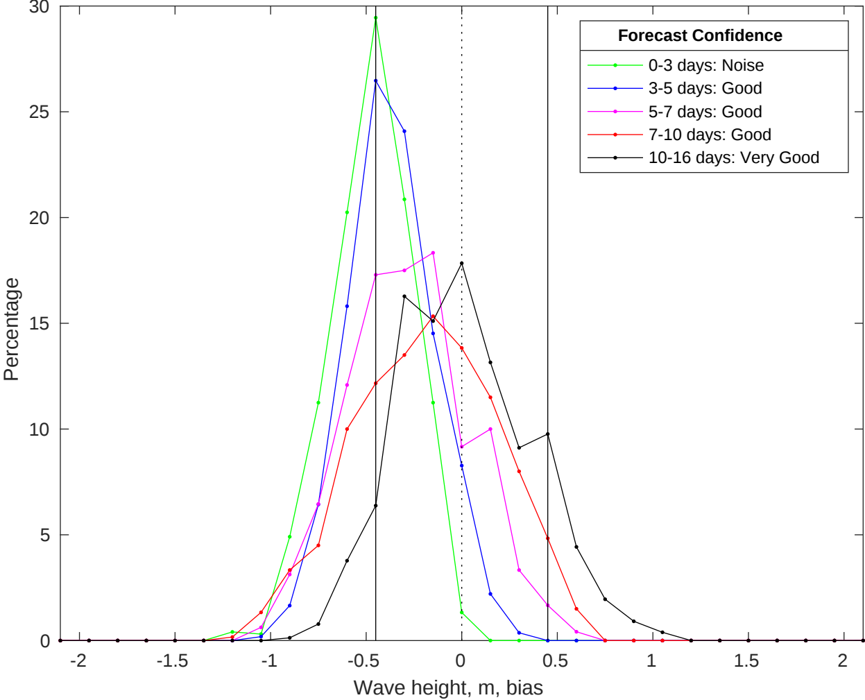
NDBC 51209 vs GFS Waves Bias Histogram: 25-Jul-2025
