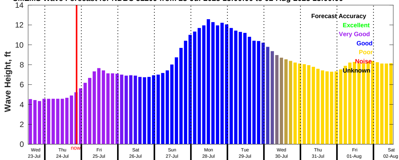
CMEMS Wave Forecast for NDBC 51209 from 23-Jul-2025 13:00:00 to 02-Aug-2025 13:00:00
