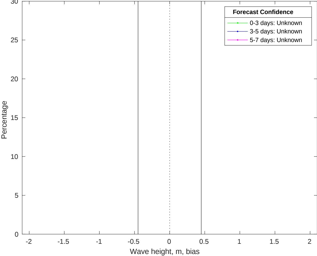
NDBC 51211 vs GFS Waves Bias Histogram: 25-Jul-2025
