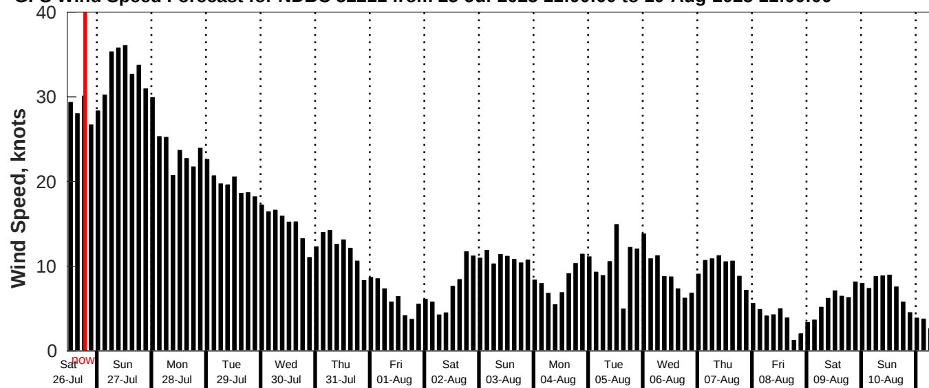
GFS Wind Speed Forecast for NDBC 52211 from 25-Jul-2025 11:00:00 to 10-Aug-2025 11:00:00
