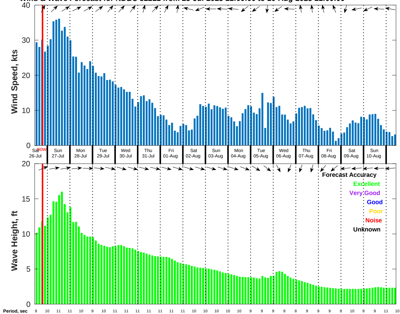
Wind & Wave Forecast for NDBC 52211 from 25-Jul-2025 11:00:00 to 10-Aug-2025 11:00:00
